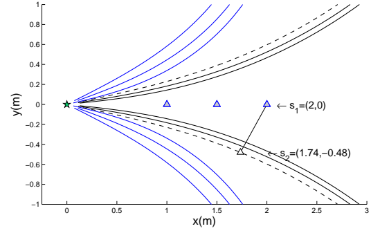
Fig. 4. Examples of the contours described by Equation (14) and (15) for a target at (0,0) (shown as a star), r_1 \in \{1, 1.5, 2\} and \lambda_d set to .01 (black lines of lesser curvature) or .05 (blue). \sigma_s was 1 and N_1 was 1. For example, if the robot first travels to the position s_1 = (2,0) and takes one measurement then it can take all remaining measurements from anywhere on the dashed curve (e.g., s_2 as labelled) to satisfy \underline{\lambda}(\mathbb{F}) = \lambda_d .
